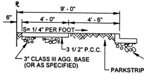
SECTION C-C RESIDENTIAL STREET
