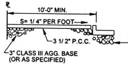
SECTION D-D HIGH DENSITY RESIDENTIAL (RETROFIT)
