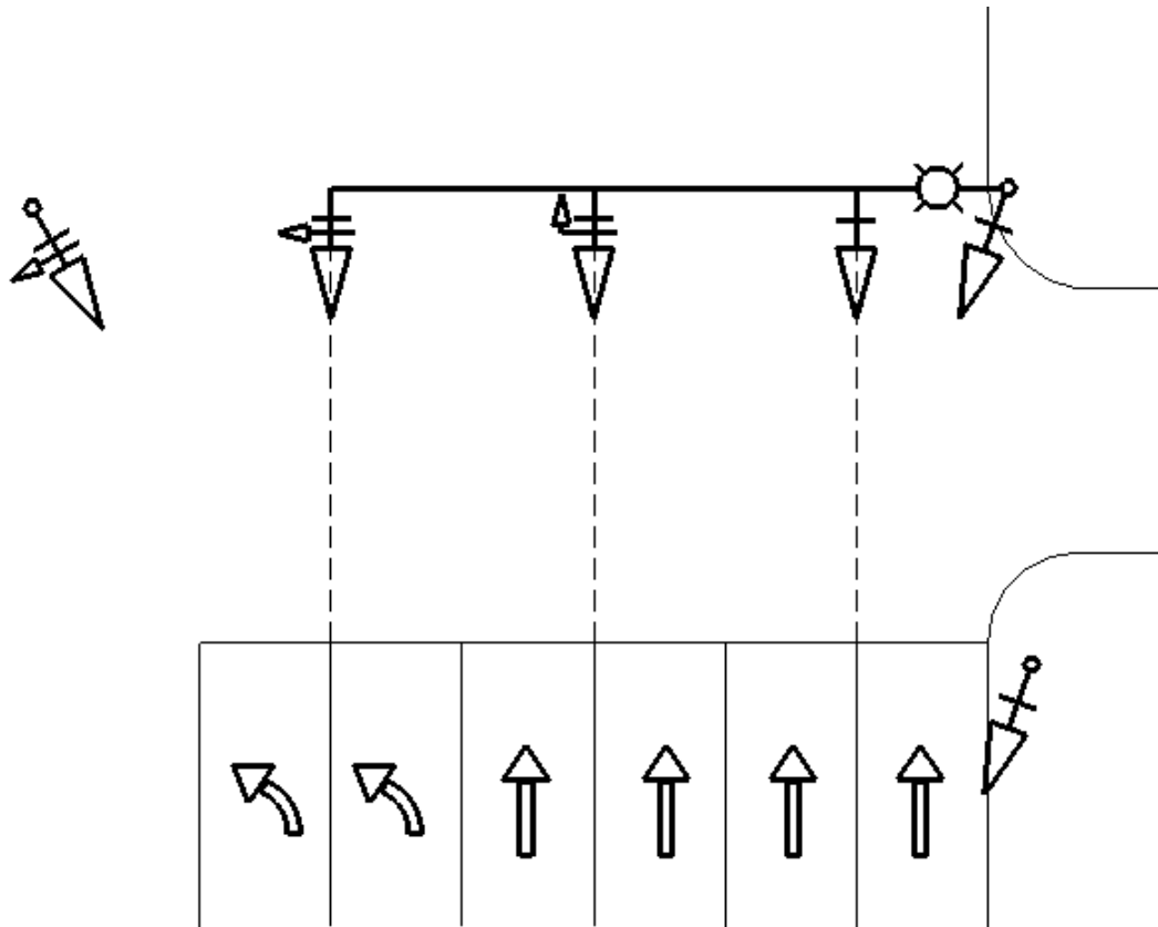
FIGURE 9: MASTARM SIGNAL FACES PLACEMENT 9
