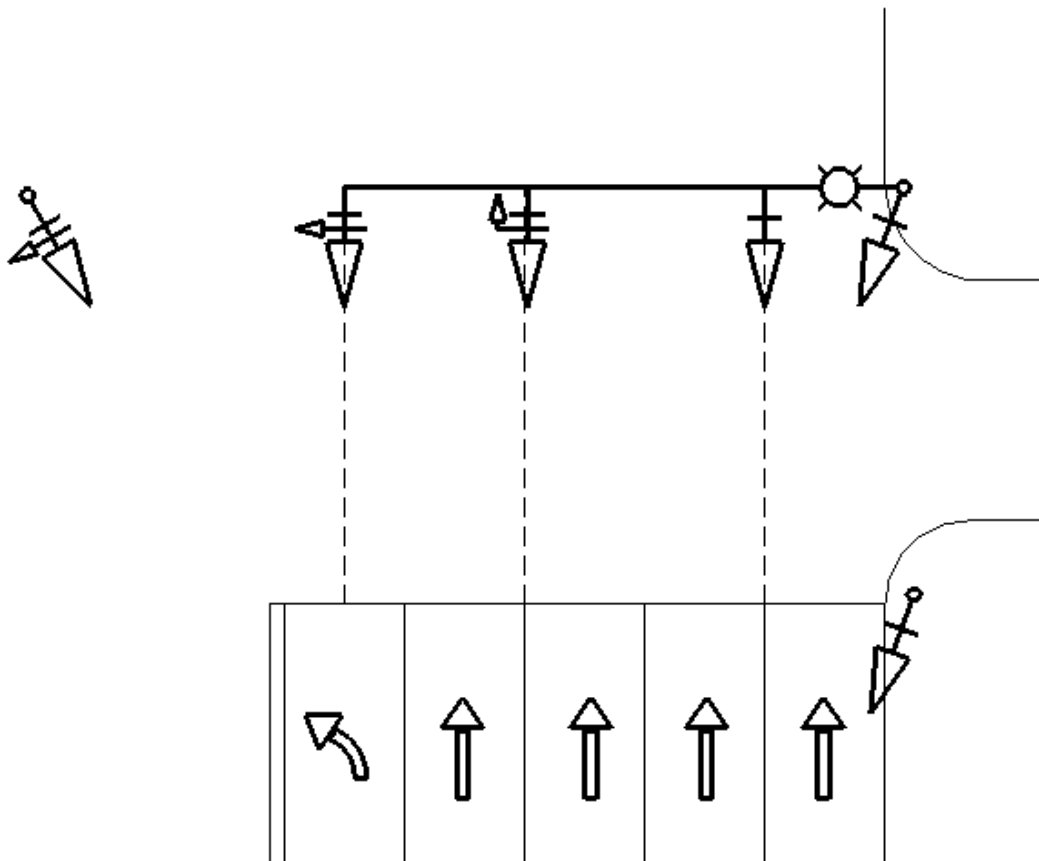
FIGURE 8 MASTARM SIGNAL FACES PLACEMENT 8
