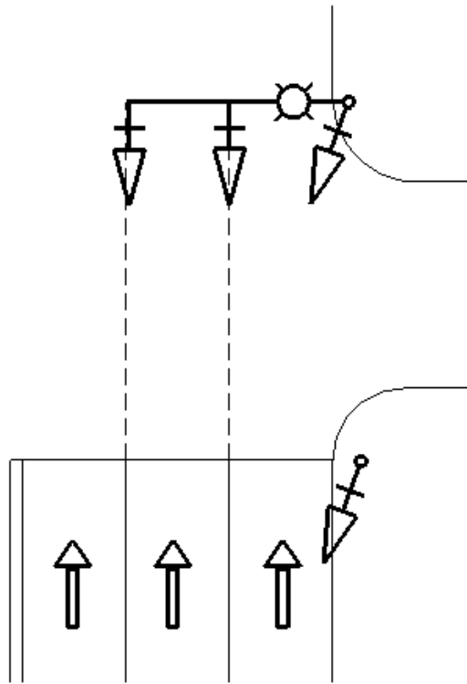
FIGURE 4: MASTARM SIGNAL FACES PLACEMENT 4
