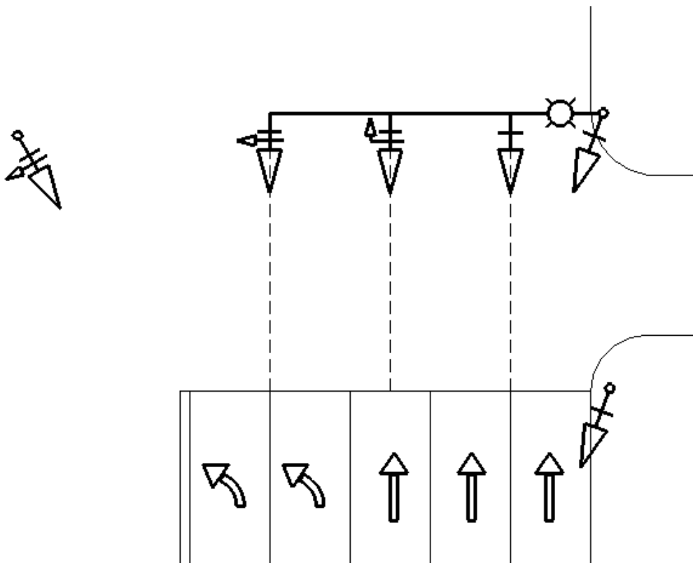
FIGURE 6: MASTARM SIGNAL FACES PLACEMENT 6
