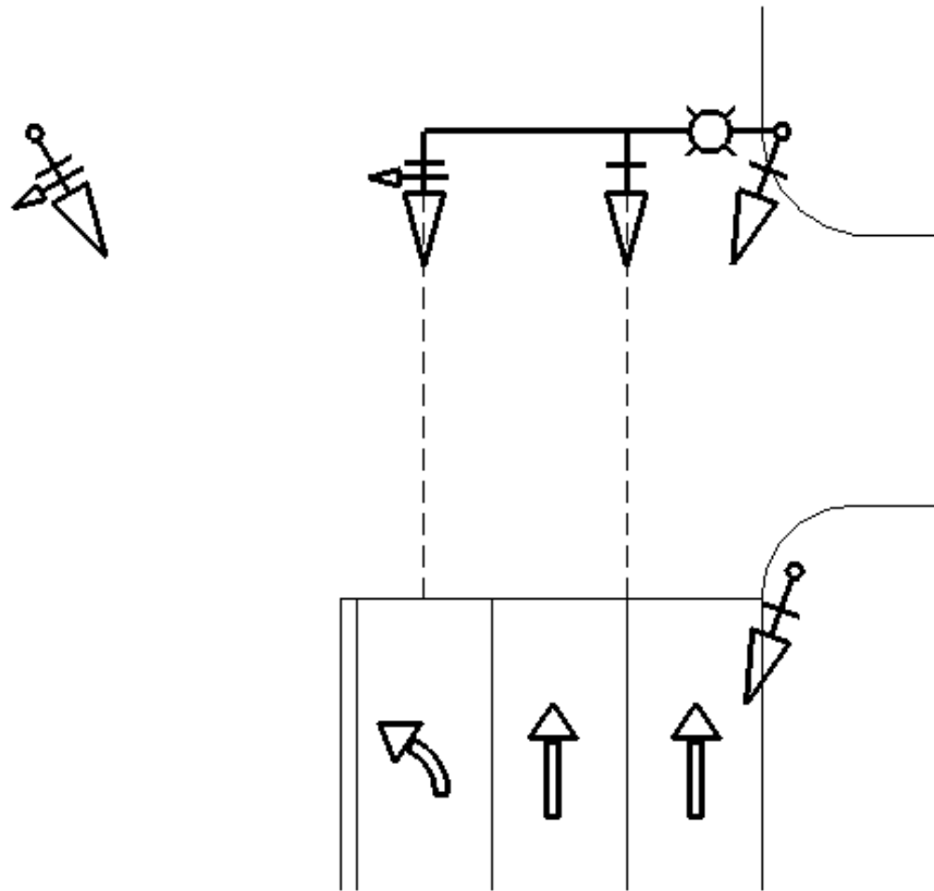
FIGURE 1: MASTARM SIGNAL FACES PLACEMENT 1
