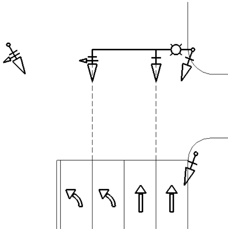
FIGURE 3: MASTARM SIGNAL FACES PLACEMENT 3
