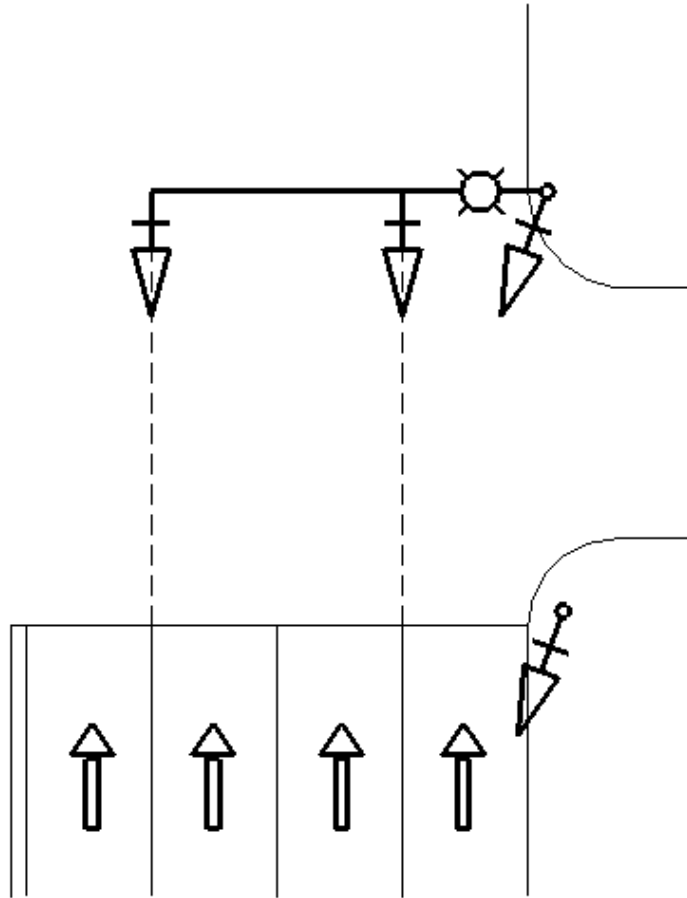
FIGURE 7: MASTARM SIGNAL FACES PLACEMENT 7
