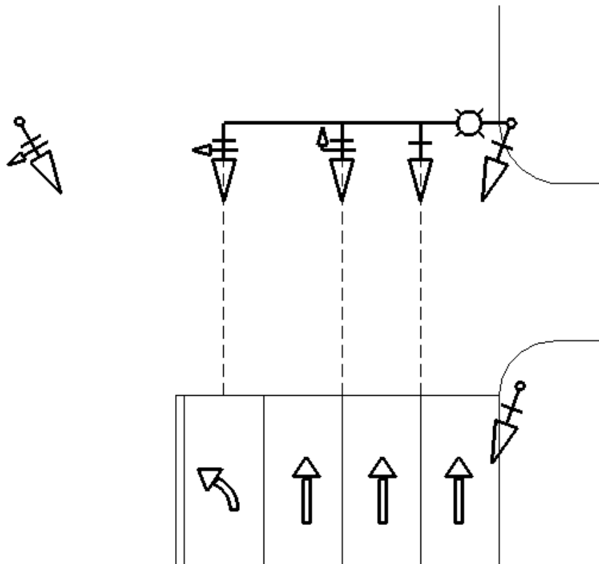
FIGURE 5: MASTARM SIGNAL FACES PLACEMENT 5
