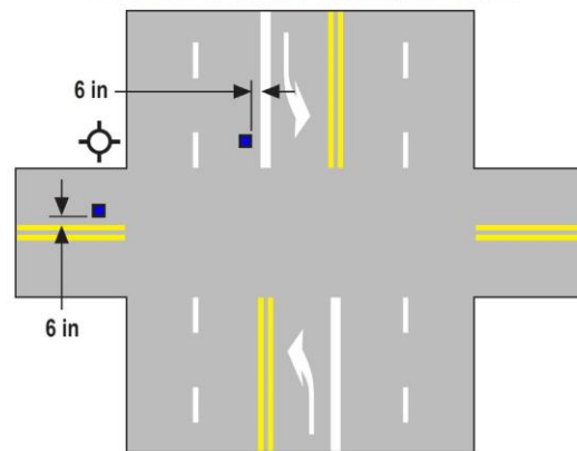
FOUR LANE STREET WITH TURN LANE AT INTERSECTION
