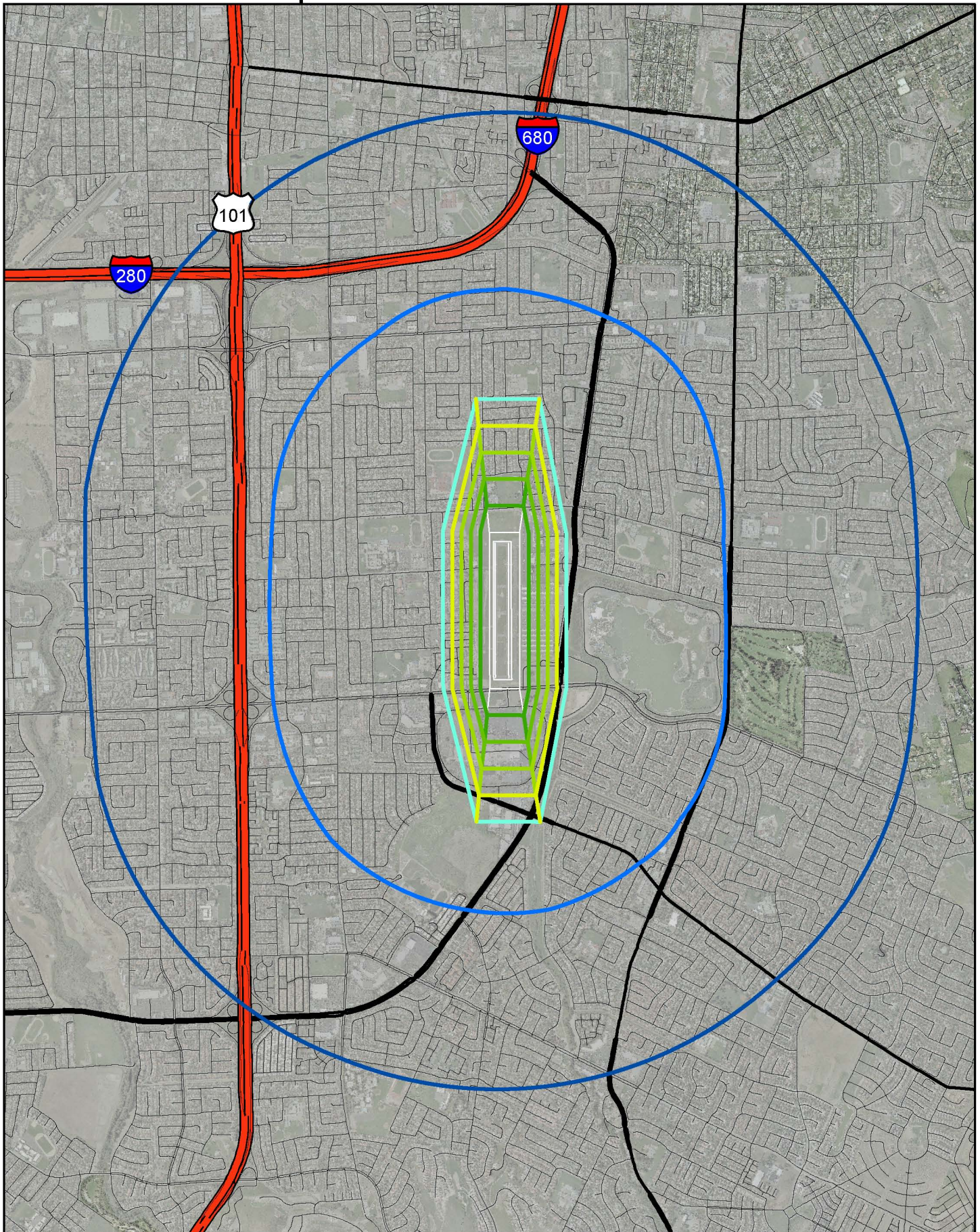
Figure 6 FAR Part 77 Surfaces
