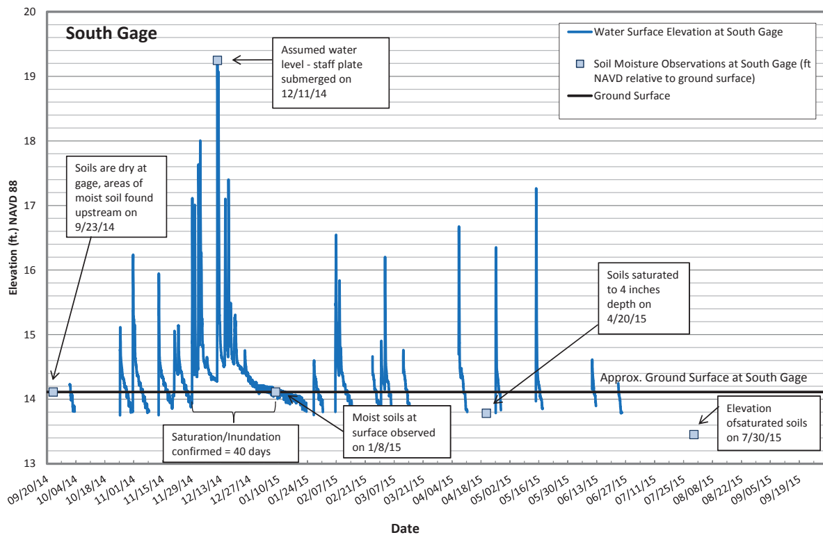
Figure 4. Annotated stage record - Wrigley Creek Mitigation Performance Monitoring, Water Year 2015, Milpitas, California Stage record for the north and south stations with storms shown by the steep spikes in stage followed by a gradual decline as the monitoring locations drain. Note that the pressure transducers are installed below the ground surface. Soil moisture observations are elevations in NAVD and should be compared to the adjacent ground surface.
