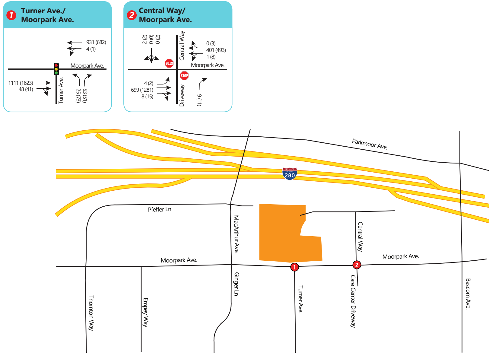
Figure 11: Background Conditions Lane Geometry, Controls and Traffic Volume
